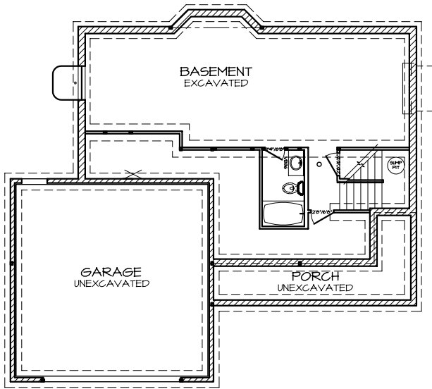
1 FOUNDATION PLAN A-3
