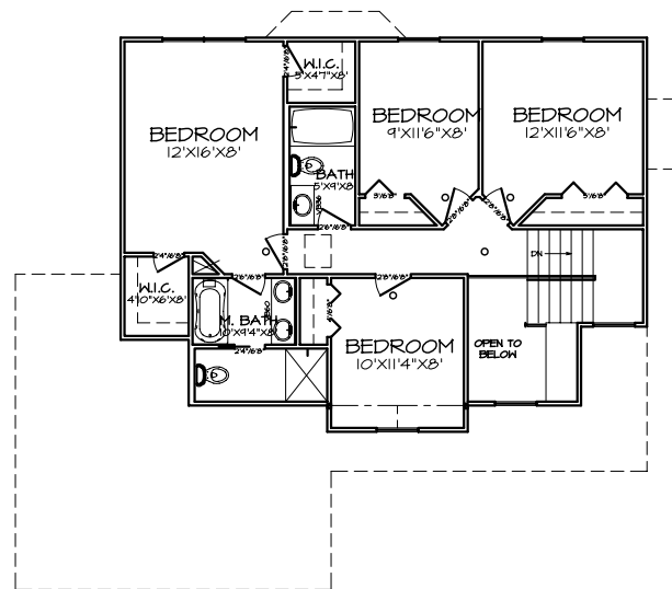
1 SECOND FLOOR PLAN A-5
